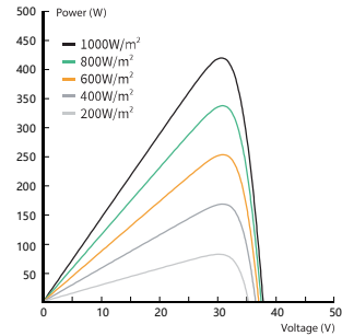
Power-Voltage Curve(420W)
